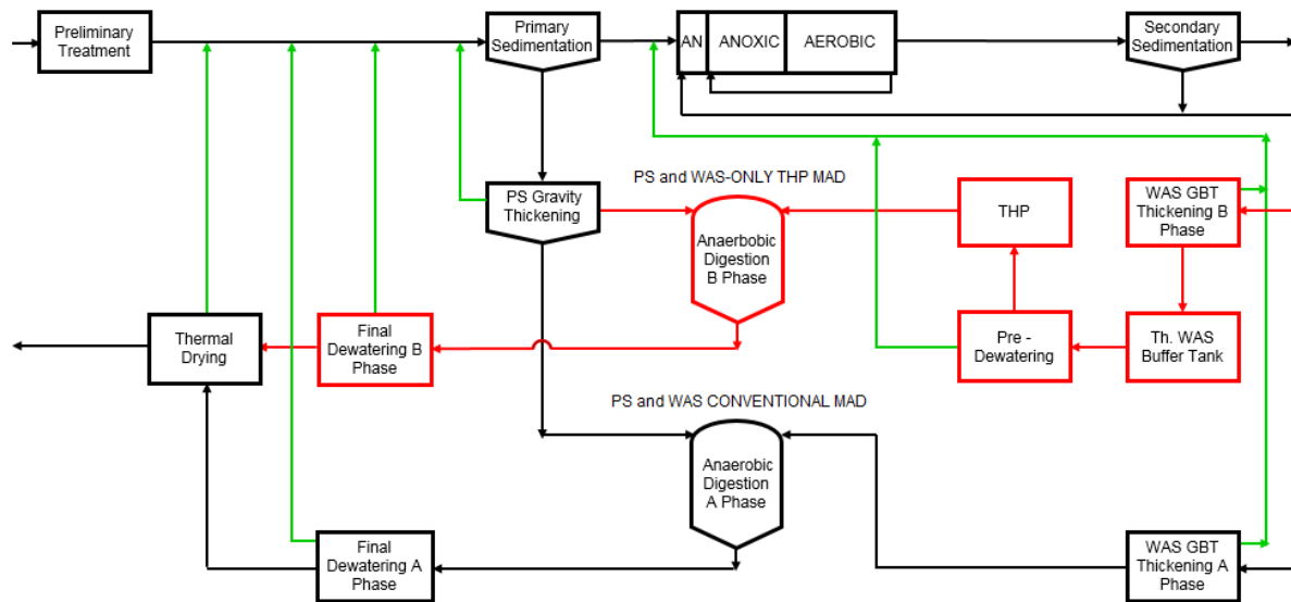
Figure 5: Simplified flow diagram of the Wastewater and Sludge treatment lines of Psyttalia WWTP. The WAS-Only treatment sludge line is highlighted in red.
