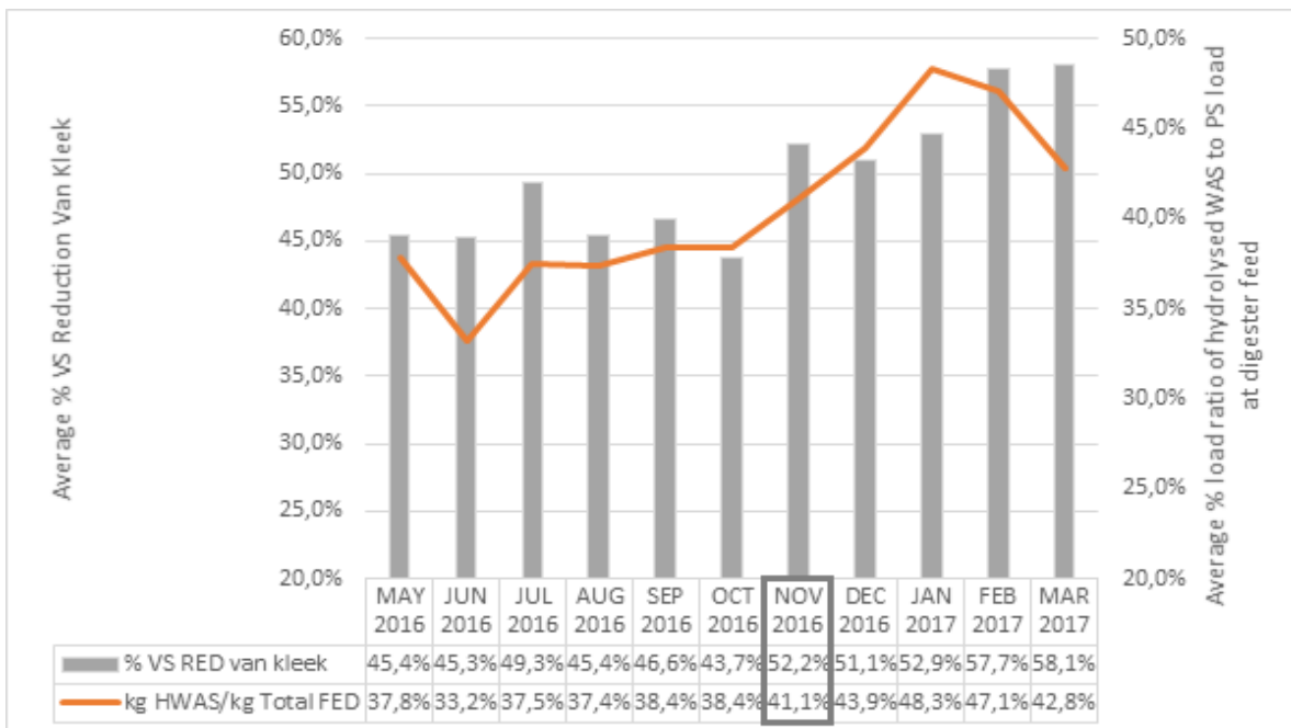
Figure 8: DS load ratio of hydrolysed WAS to total DS load at digester feed and calculated VS reduction
