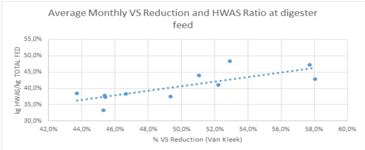
Figure 9: Relationship of the DS load ratio of hydrolysed WAS to total DS load at digester feed and calculated VS reduction
