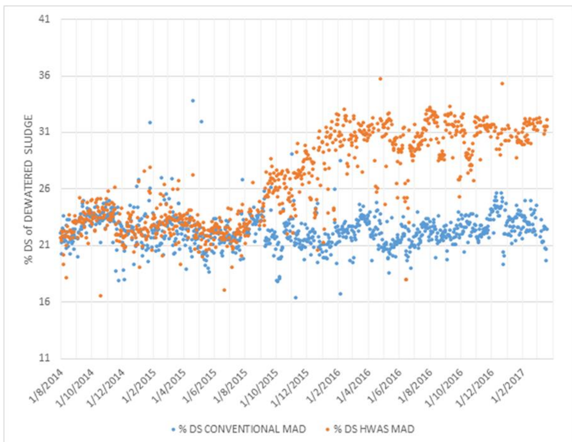
Figure 11: Dryness in %DS of dewatered digested sludge, for Phase A (conventional) and Phase B (THP) digesters
