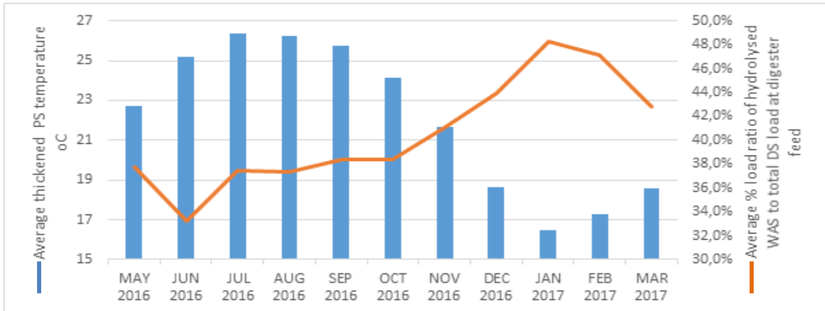
Figure 7: DS load ratio of hydrolysed WAS to total DS load at digester feed and thickened PS stream temperature
