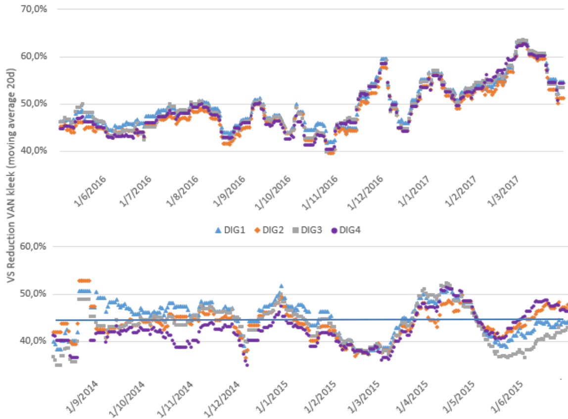
Figure 6: Calculated VS Reduction (Van Kleeck) for periods before (8/2014-7/2015) and after (5/2016-3/2017) the operation of the WAS-Only THP
